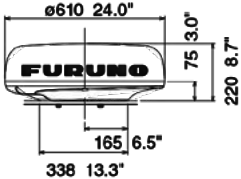
DRS4D-NXT 24" Radome Radar Sensor 7.3 kg 16.1 lb
