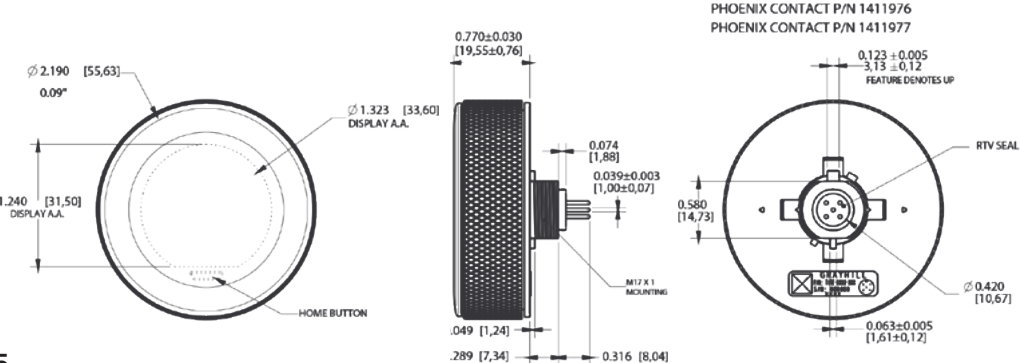
TEU001B/S Touch Encoder Unit (option, U.S. and Canada only) 0.12 kg 0.26 lb
