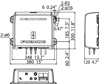
DFF3-UHD Network Fish Finder 3.8 kg 8.4 lb
