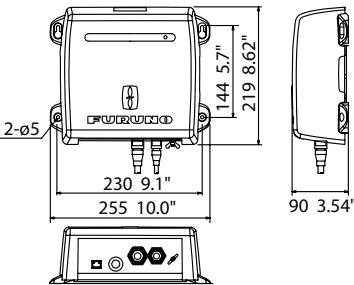
BBDS1 Network Fish Finder/Bottom Discrimination Sounder 1.3 kg 2.9 lb
