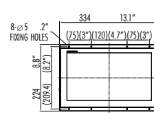
Flush Mount
