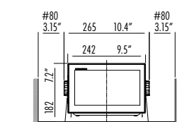
Bracket Mount
