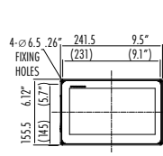
Flush Mount
