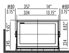
Bracket Mount
