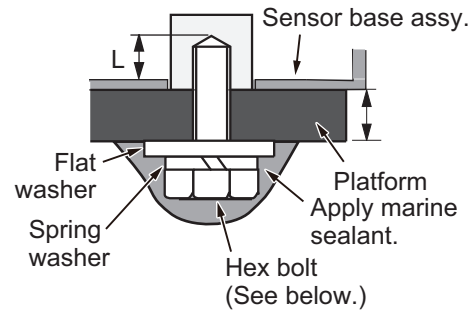
Platform thickness and bolt to use
