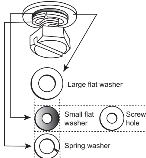
Default position of bolt and washer
