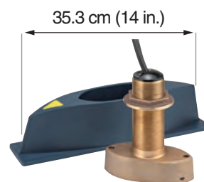
Thru-hull mount transducer B54 or SS54 Transom mount transducer TM54
